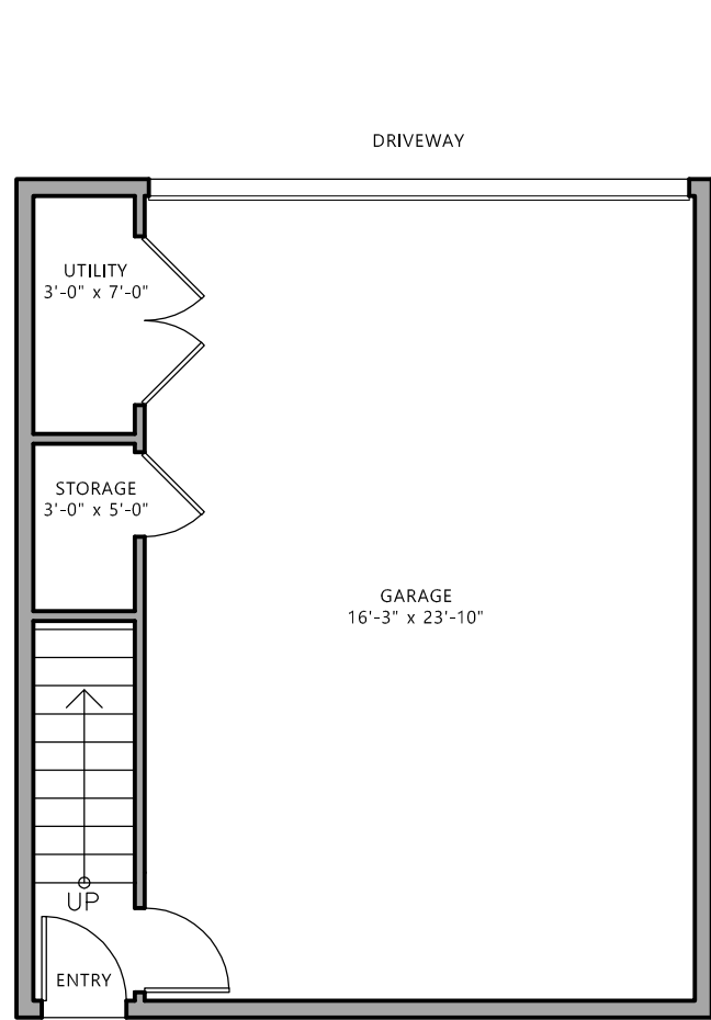
GARAGE LEVEL: 46 SF
