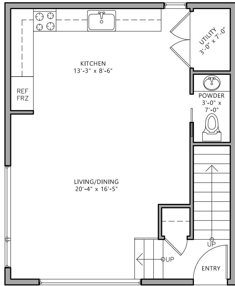
GROUND LEVEL: 511 SF
